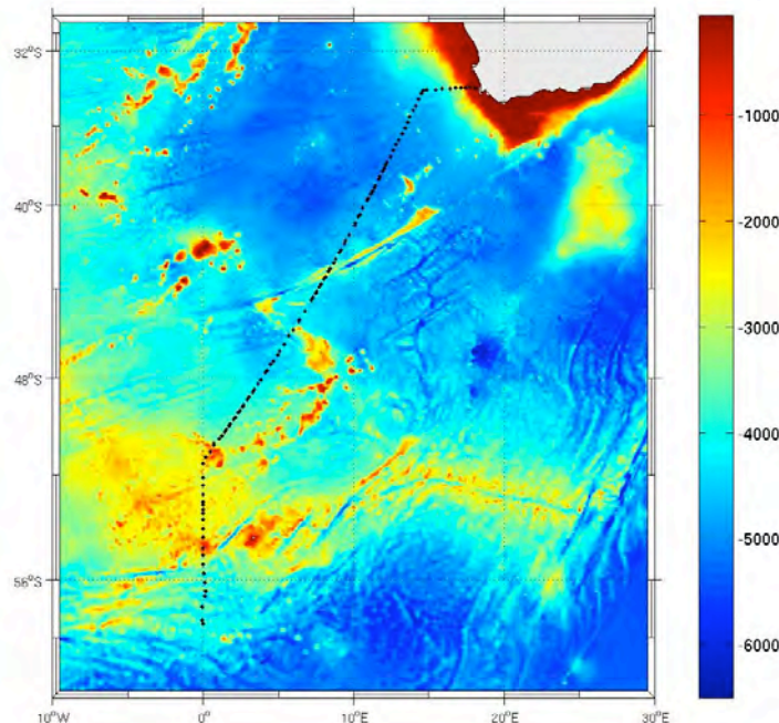
Figure 14 Position of XBT stations (black dots) occupied during the BONUS-GOODHOPE survey. The station positions are overlaid onto the bathymetry (in meters) of the region.
