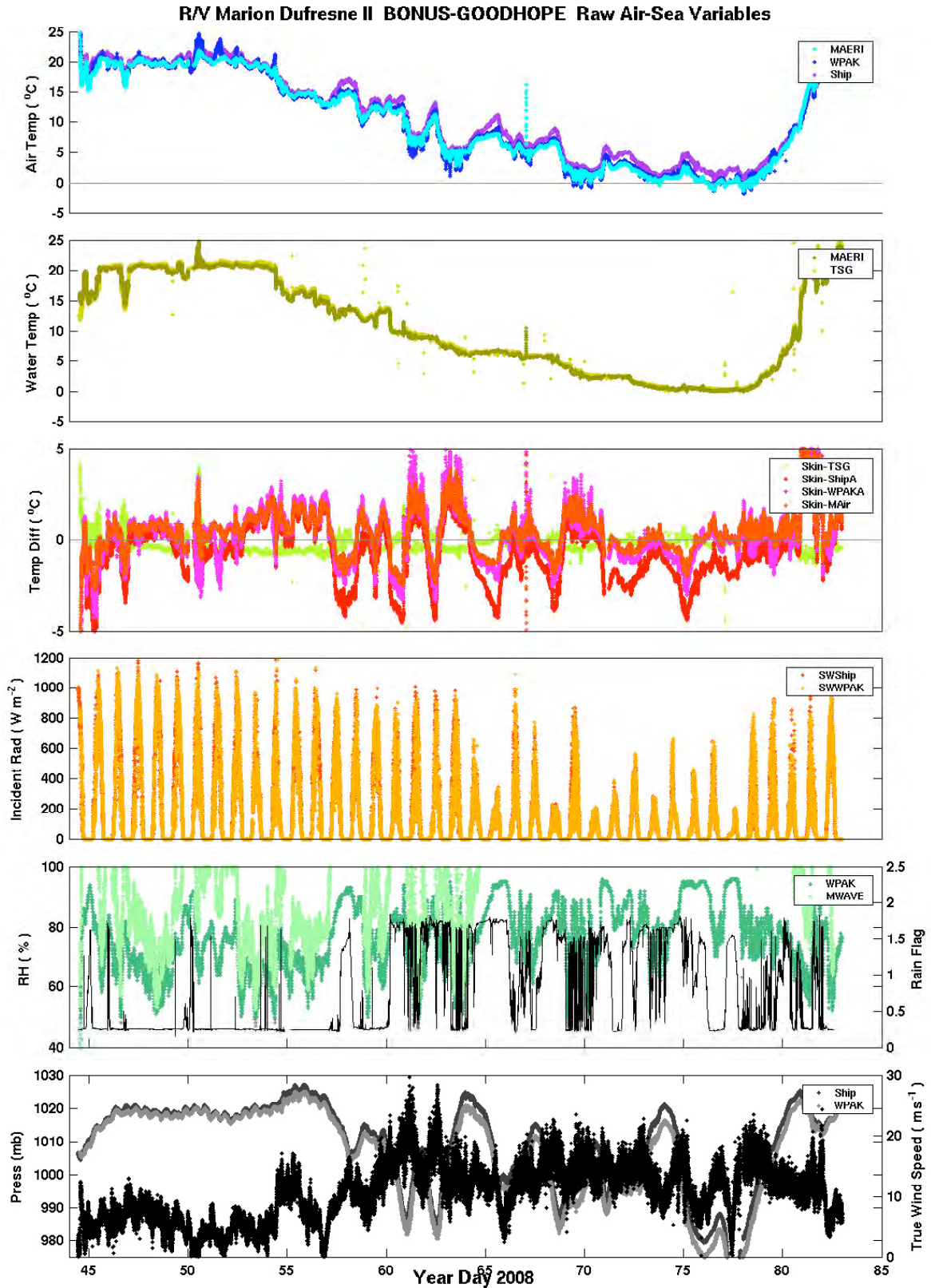
Figure 35 Time series of the merged data sets, including meteorological, radiative, and radiometric variables.
