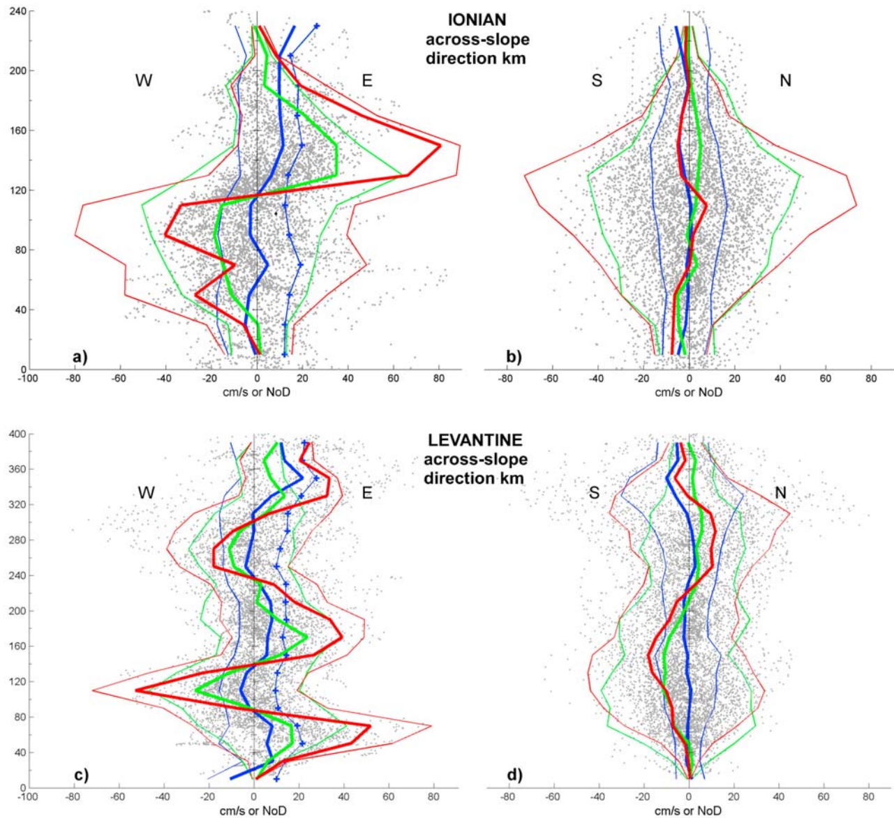
Figure 2. (a, c) E and W components and (b, d) N and S components in the Ionian and in the Levantine, respectively, plotted on the x-axis (cm/s) as a function of distance in the across-slope direction (y-axis, km). In all plots: available data are plotted as grey dots; thin lines link points representing 20-km averages of the Number of Data (NoD, green, x-axis numbers to be multiplied by 10), the mean (blue), the sum (red, x-axis numbers to be multiplied by 100); thick lines represent net E–W and N–S values.
