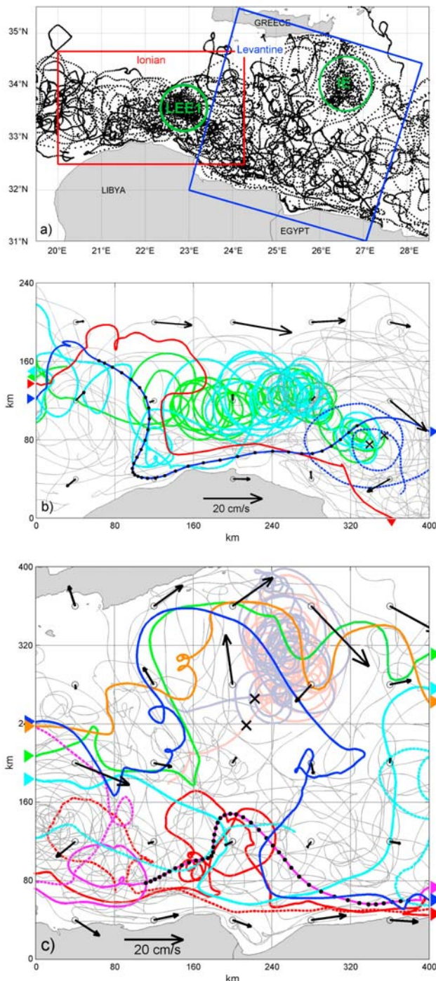
Figure 1. (a) The available trajectories in the study area, highlighting the (b) Ionian (red rectangle in Figure 1a) and (c) Levantine (blue square in Figure 1a) domains; the relatively motionless Ierapetra-05 and Ierapetra-06 (IE) eddies as well as the westward drifting LEE-1 eddy are located as in February 2006. In Figures 1b and 1c all available trajectories are in grey; the triangles specify the beginning and end of the coloured trajectories at the borders of the domains and the crosses specify launching locations in their interiors; parts of the coloured trajectories prior to or after crossing the domains are dashed; the 10-day largest eastward displacements are marked by (41) positions (black dots) plotted at 6-h intervals; the mean currents in each 80 km by 80 km box originate at the centre.
